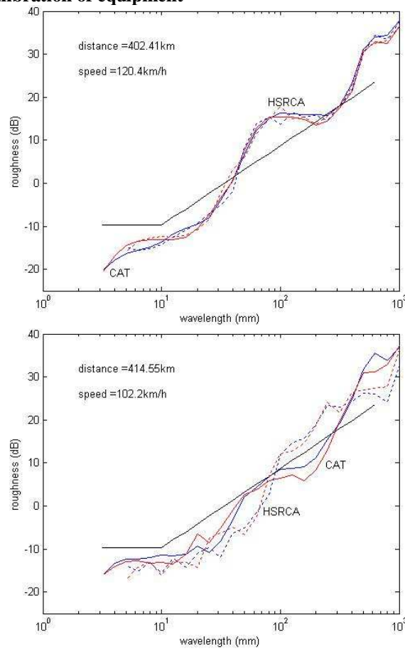
Fig. 4: Correlation of HSRCA and direct measurements of railhead roughness at reference sites
