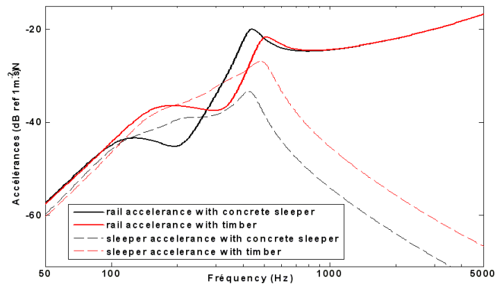
Fig. 3: rail and sleeper accelerances, for concrete and wooden sleeper track. Track modelled with a Timoshenko beam continuously supported with a double stiffness layers: rail UIC60, ballast stiffness equal to 100 \text{ MN/m}^2 , railpad stiffness equal to 300 \text{ MN/m}^2 , sleeper masses: concrete: 245 \text{ kg} timber: 96 \text{ kg}
