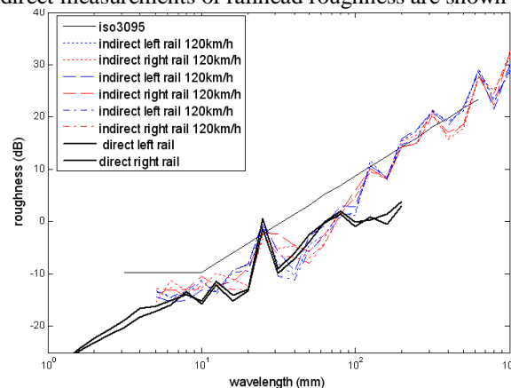
Fig. 5: Repeatability of measurements at 120km/h, and comparison of HSRCA and direct measurements of railhead roughness, test site 3
