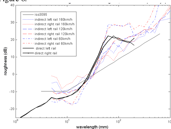
Fig. 6: Effect of speed on HSRCA measurements and comparison of HSRCA and direct measurements of railhead roughness, test site 2
